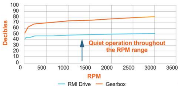
Db @ 1 Meter
