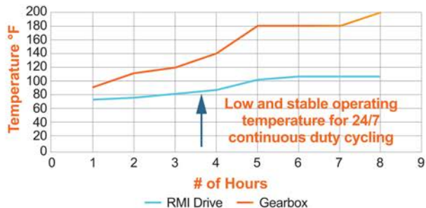
Operating Temperature @ 72° Ambient
