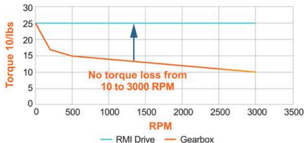
Torque Curve at set RPM
